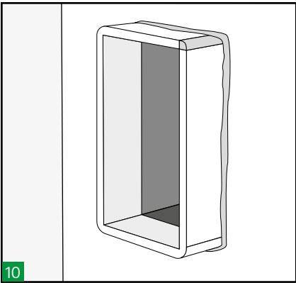
Weld frame in position in accordance with Rectangular frame HMX welding instructions and seal the frame in accordance to rectangular system installation guide.
